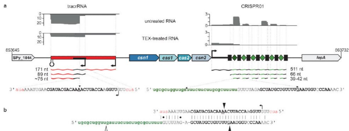
Figure 2. Identification of tracrRNA in S. pyogenes as reported in [27]. a. Differential RNA sequencing (dRNA-seq) reveals expression of tracrRNA and crRNAs. Sequence reads of cDNA libraries of RNA are shown on top. Below is the genomic organisation of tracrRNA and CRISPR01/Cas loci. Red bar: tracrRNA is encoded on the minus strand and detected as 171-, 89- and ~75-nt tracrRNA species. Black rectangle inside the red bar: 36-nt sequence stretch complementary to CRISPR01 repeat. The pre-crRNA is encoded on the plus strand. Black rectangles: CRISPR01 repeats; green diamonds: CRISPR01 spacers; 511, 66 and 39-42 nt: pre-crRNA and processed crRNAs. b. Base-pairing of tracrRNA with a CRISPR01 repeat is represented. Cleavages observed by dRNA-seq and leading to the formation of short overhangs at the 3' ends of the processed RNAs are indicated by two black triangles.
