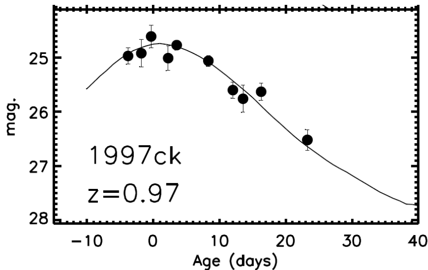
Figure 1. One of the high redshift supernovae of type Ia for which the HST collaboration [27] could measure the magnitude, i.e., the luminosity, both before and after the peak luminosity.
